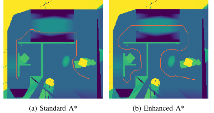
Fig. 7: Standard A* path versus enhanced A* path.
