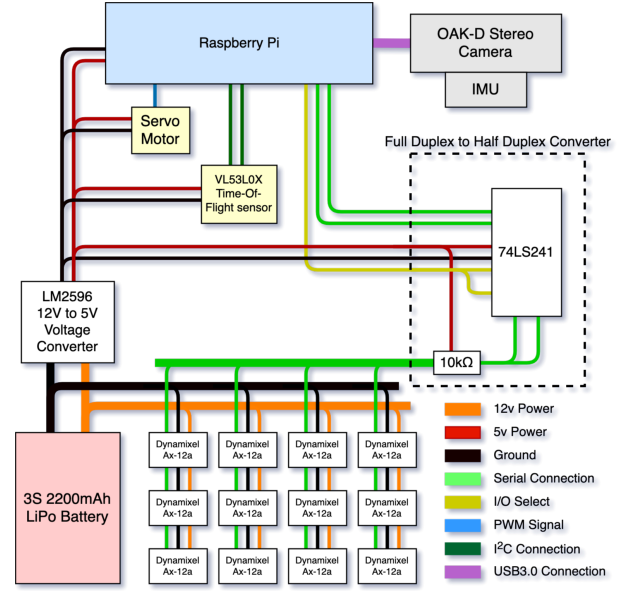
Fig. 2: Schematic of the quadruped robot.
